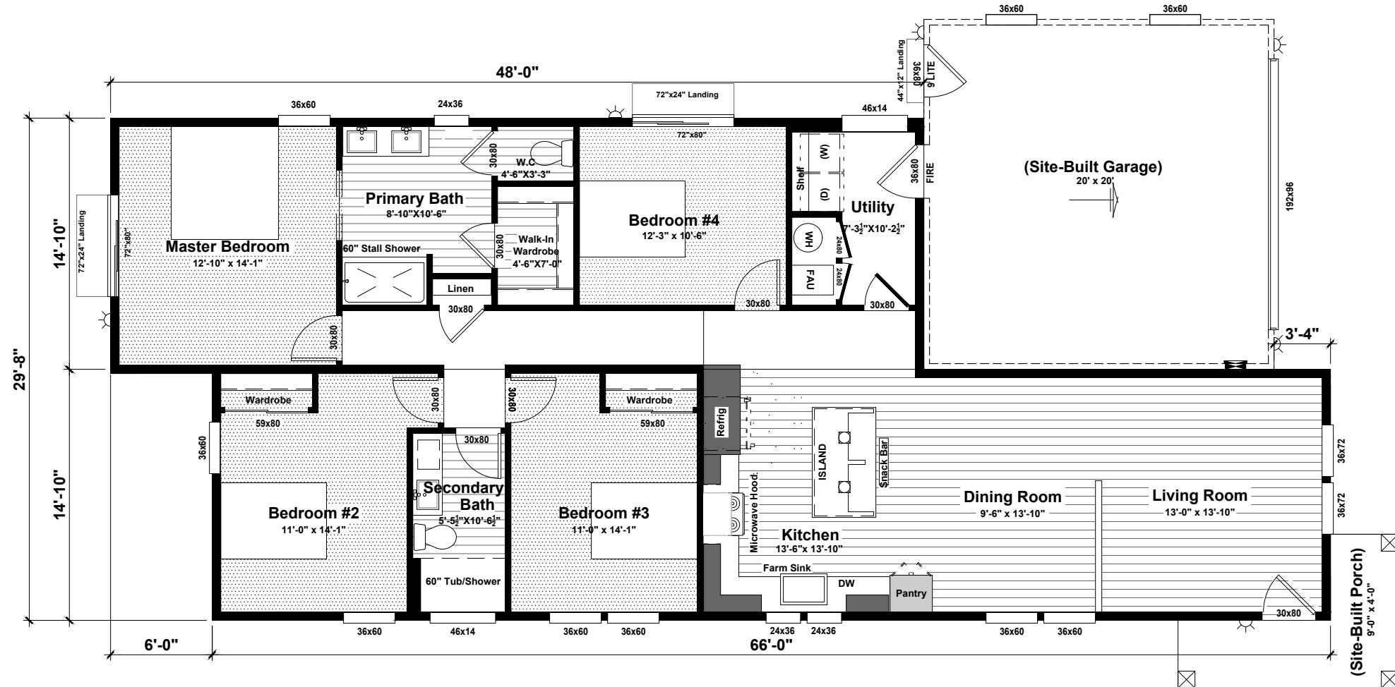
Plan 1A 4 Bed | 2 Bath | 1,691 Sq. Ft.
