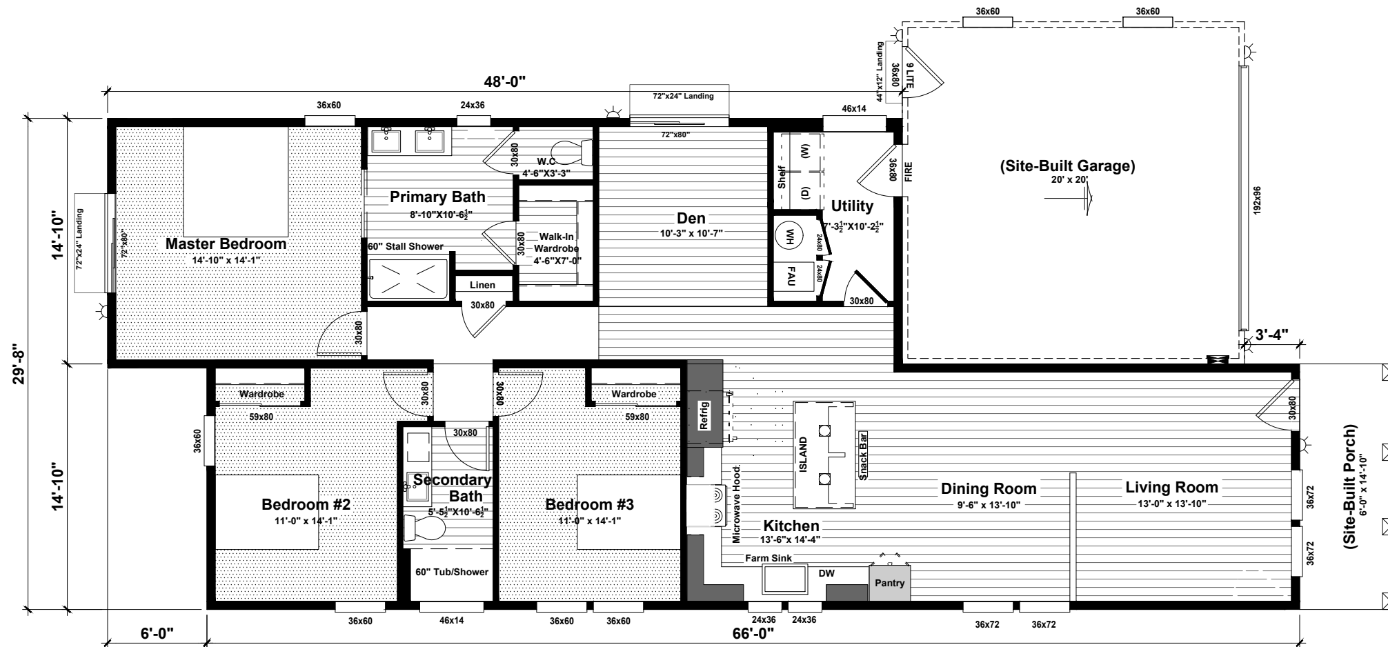
Plan 3A 3 Bed | 2 Bath | 1,691 Sq. Ft.
