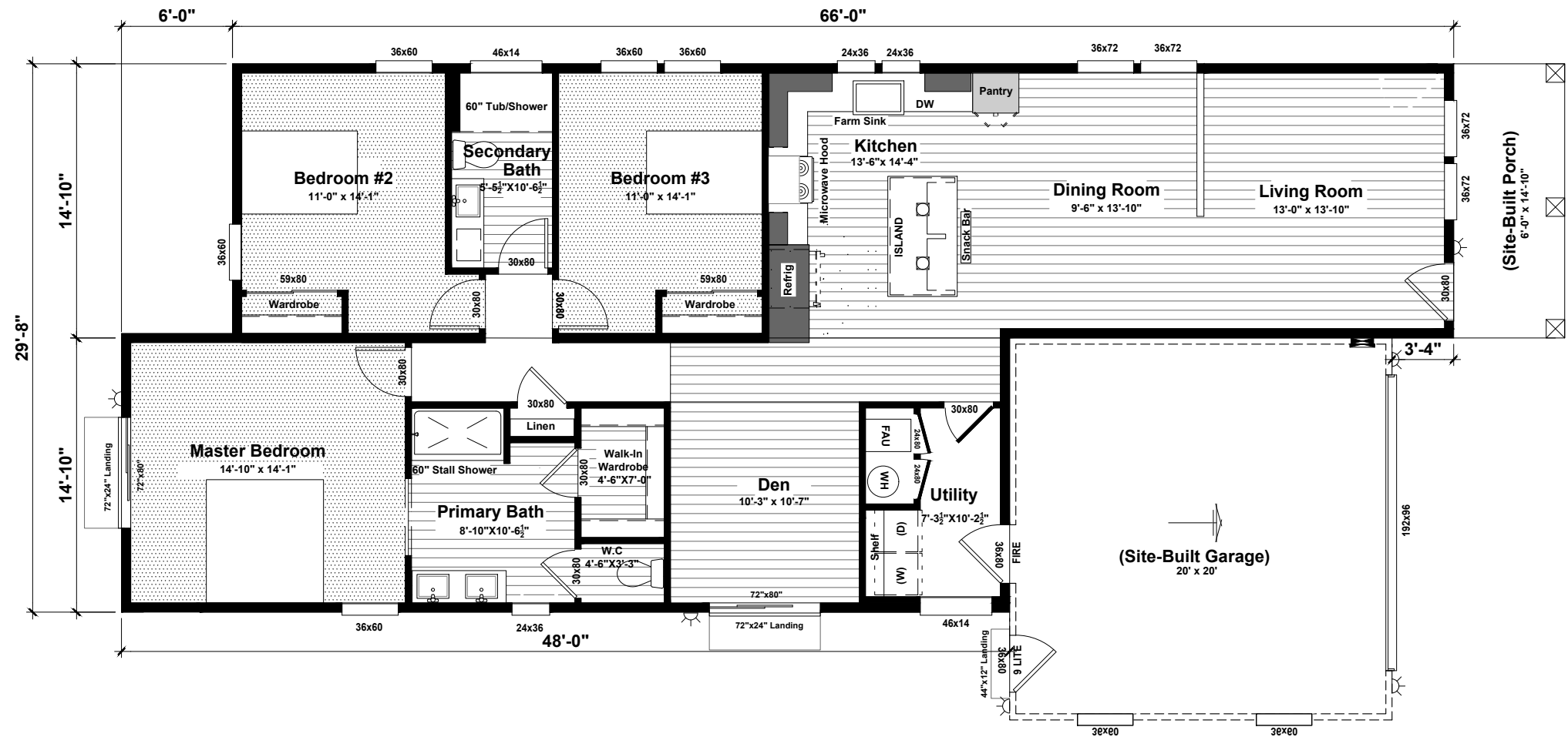
Plan 4A 3 Bed | 2 Bath | 1,691 Sq. Ft.
